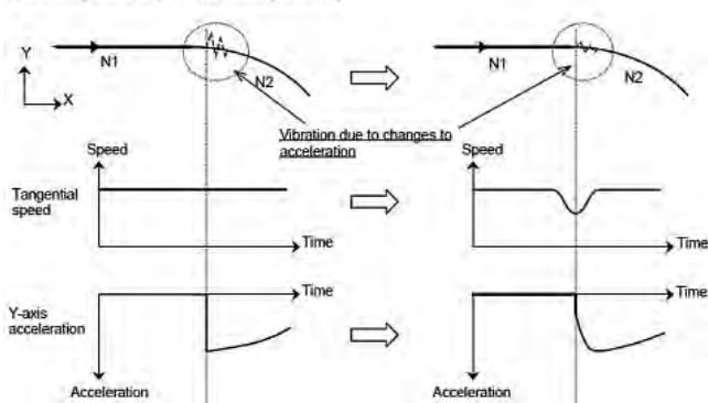
Linear interpolation (N1) → circular interpolation (N2)
