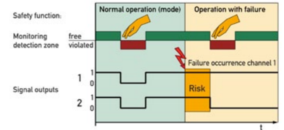
Fig. 1: View of a redundant system according to ISO 13849-1
