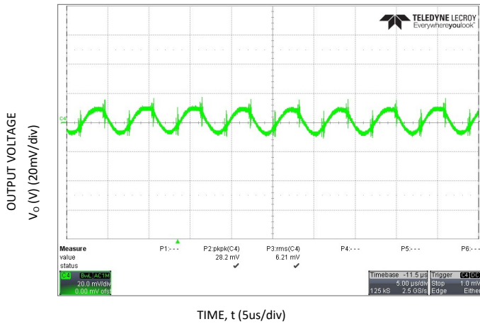
Figure 3. Typical output ripple and noise (Co = 500uF Ceramic + 500uF PosCap Oscon, Vin = 56V, Io = Io,max).
