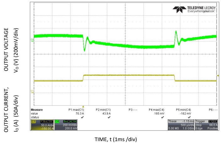
Figure 4. Dynamic Load Response, di/dt=1A/us; Vin=Vin,nom; TA=25°C; Load Change from Io = 50% to 75% of Io,max; Co = 4000uF Ceramic;
