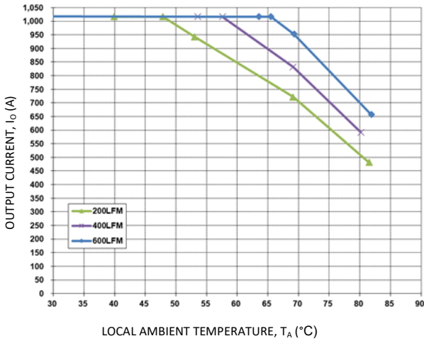
Figure 17. Output Current Derating for the Base plate QBDS095A10R6-H+0.6" Heat Sink; Airflow Direction for Vout to Vin(Worst) orientation; Vin = 50V.
