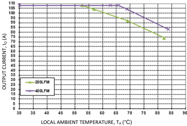
Figure 17. Output Current Derating for the Base plate QBDS108A0B-H+0.6" Heat Sink; Airflow Direction for Vout to Vin(Worst) orientation; Vin = 50V.
