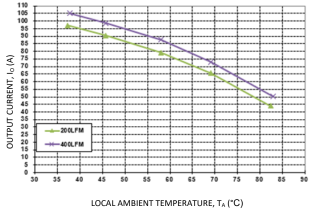
Figure 16. Output Current Derating for the Base Plate QBDS108A0B-H; Airflow Direction for Vout to Vin(Worst) orientation; Vin = 54V.
