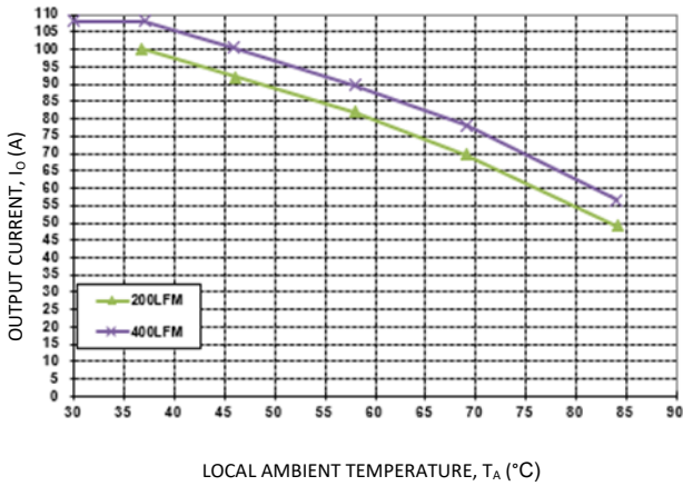
Figure 15. Output Current Derating for the Base Plate QBDS108A0B-H; Airflow Direction for Vout to Vin(Worst) orientation; Vin = 50V.
