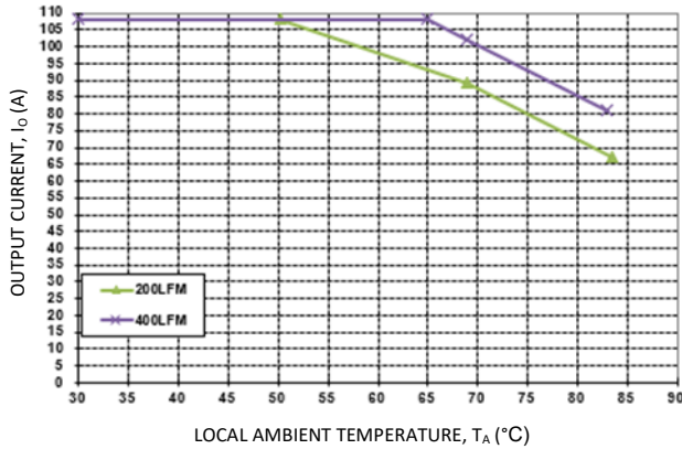
Figure 18. Output Current Derating for the Base plate QBDS108A0B-H+0.6" Heat Sink; Airflow Direction for Vout to Vin(Worst) orientation; Vin = 54V.
