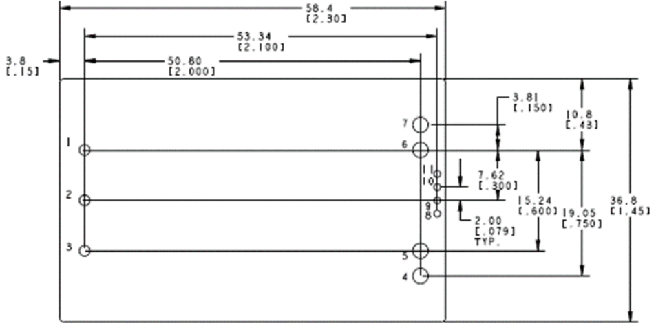
TOP VIEW
