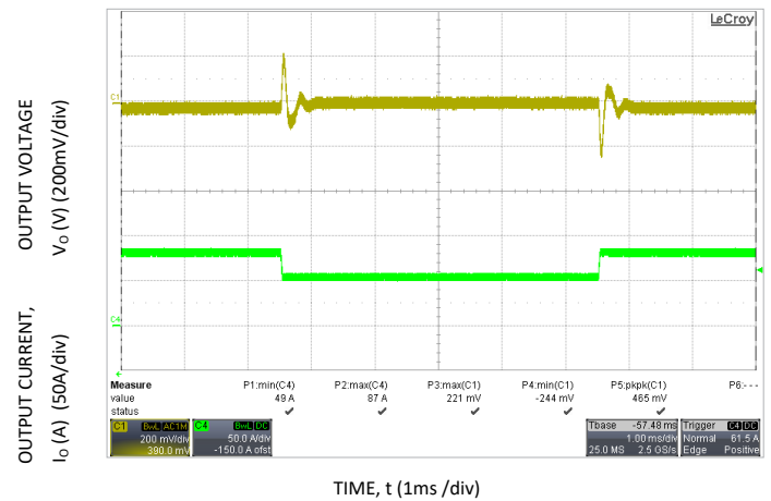
Figure 4. Dynamic Load Response, di_o/dt=1\text{A}/\mu\text{s} ; V_{in}=V_{in,nom} ; T_A=25^\circ\text{C} ; Load Change from I_o = 50\% to 75\% of I_{o,max} ; C_o = 5200\mu\text{F} Ceramic;
